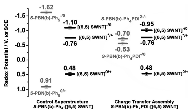
Figure 1. Energy level diagram highlighting the experimentally determined redox potentials of the polymer and SWNT components of S -PBN(b)-Ph 5 -[(6,5) SWNT] and S -PBN(b)-Ph 4 PDI-[(6,5) SWNT] superstructures. The [(6,5) SWNT] */+ excited-state reduction potential was determined from the (6,5) SWNT E_{00} \rightarrow E_{11} optical band gap ( \Delta E_{11} = 1.24 eV) and its ground state oxidation potential ( E^{0/+} = 0.48 V). In the potentiometric experiments used to determine these redox potentials, the ferrocene/ferrocenium (Fc/Fc + ) redox couple ( E_{1/2}^{0/+} = 0.48 V vs. SCE) was used as an internal standard. Experimental conditions: CH 2 Cl 2 solvent, 0.1 M n Bu 4 NPF 6 , T = 20^\circ\text{C} . Tabulated potentiometric data are available in the Supporting Information.
