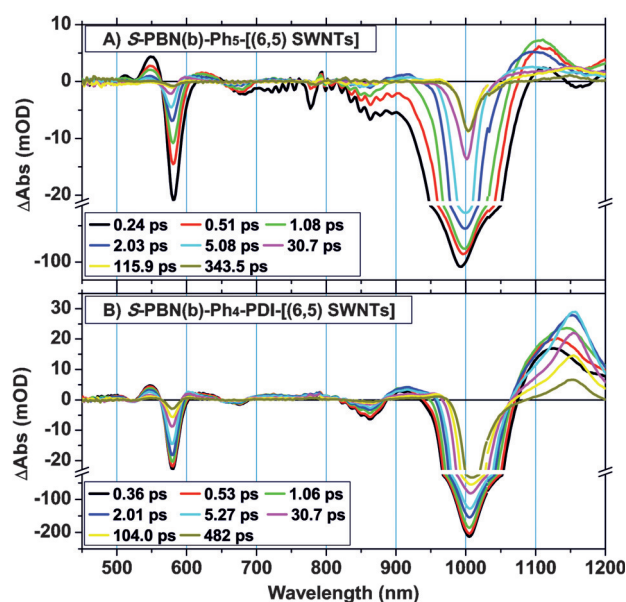
Figure 2. Representative transient absorption spectra recorded for A) S -PBN(b)-Ph 5 -[(6,5) SWNT] and B) S -PBN(b)-Ph 4 PDI-[(6,5) SWNT] samples dispersed in 3:7 MeOH/D 2 O at the time delays noted. Experimental conditions: [(6,5) SWNTs] ca. 90.3 nm; SWNT length = 700 \pm 50 nm; argon atmosphere; optical path length = 2 mm; \lambda_{\text{ex}} = 1000 nm; pulse energy = 180 nJ/pulse; temperature = 20^\circ\text{C} ; magic angle polarization.
